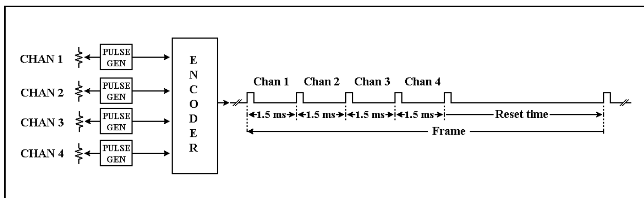
Figure 2 - Encoder timing
